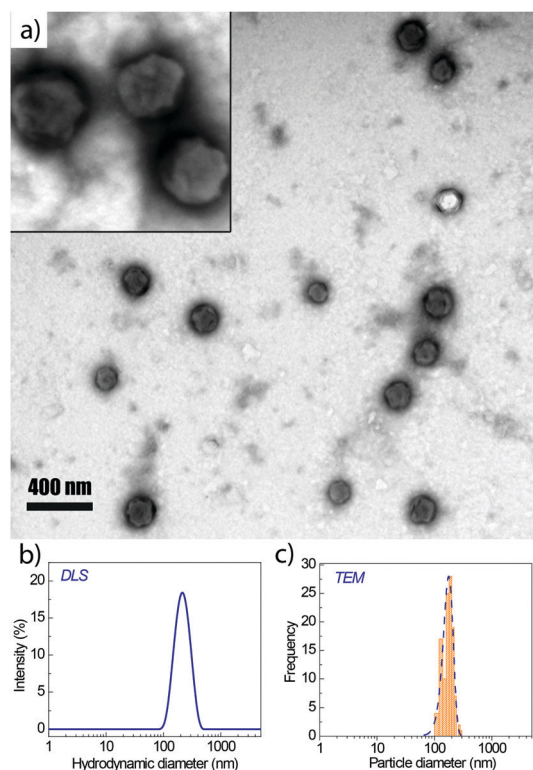
Fig. 1 TEM image of PEI/FeOx-PSAs (a). Inset area: 520 nm × 520 nm. Particle size distributions obtained by DLS (b) and TEM (c).
