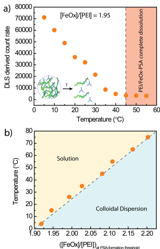
Fig. 4 Temperature response. (a) DLS temperature-trend measurement of a PEI/FeOx-PSA sample with [(\text{FeOx})]/[(\text{PEI})] = 1.95 at different temperatures, starting at 5 °C. (b) [(\text{FeOx})]/[(\text{PEI})] (mg/ml) ratio at which the transition from a molecular solution to a colloidal dispersion is observed (PSA-formation threshold) at different temperatures.
